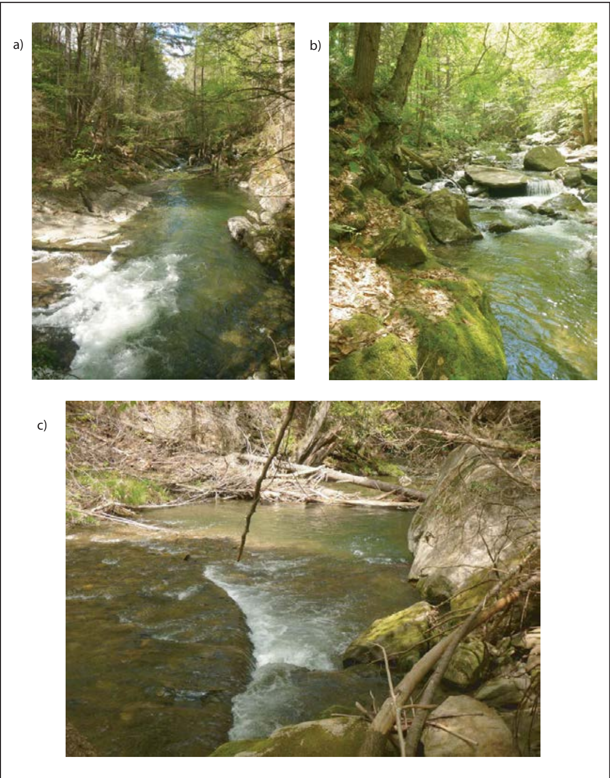
Lower Bear River Conservation Area. The a) bedrock cascade, b) boulder step-pool, and c) cobble riffle-pool stream morphologies of the lower Bear River represent a relatively natural reference condition with little evidence of past human manipulation.
